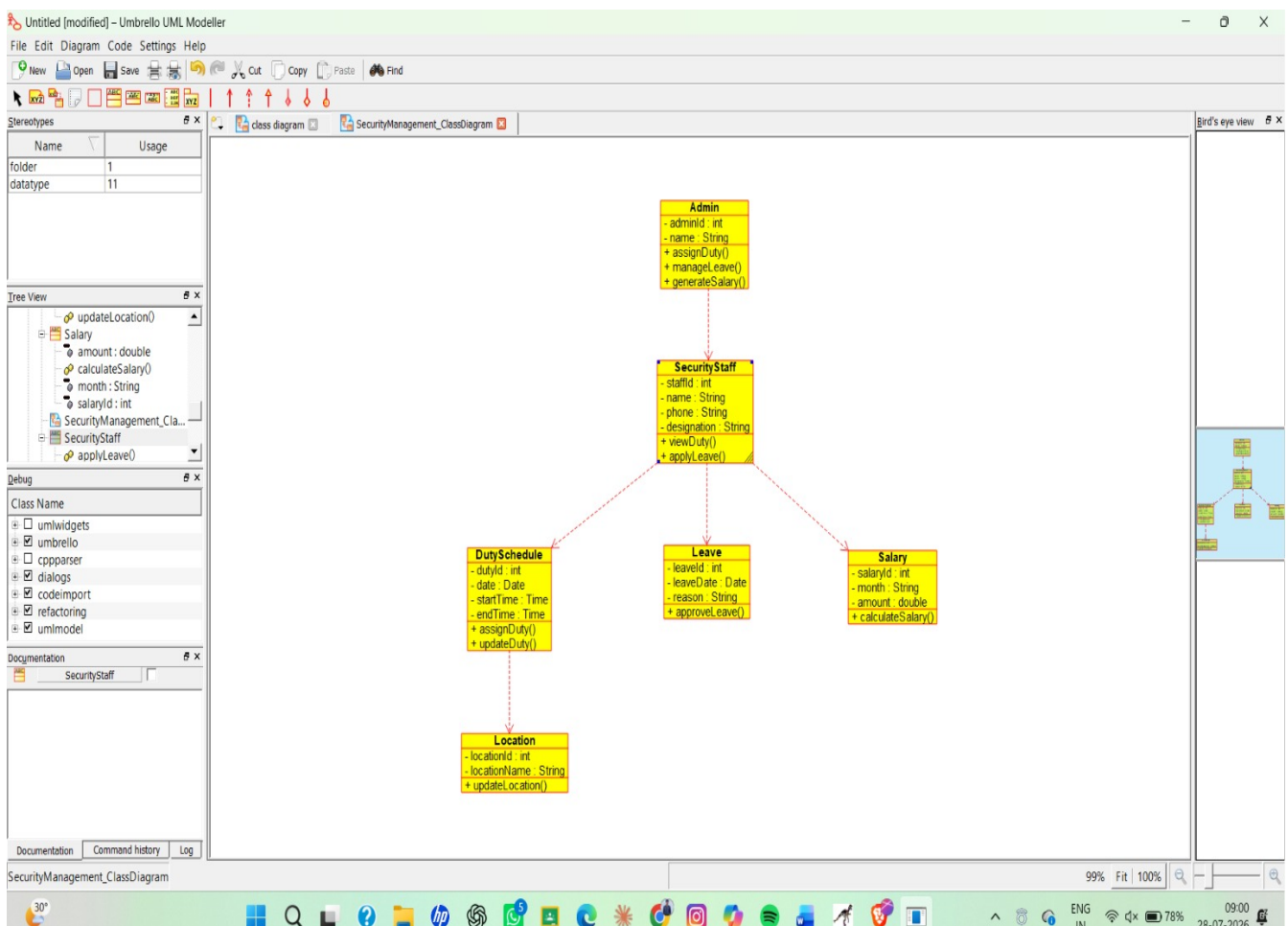
Figure 1: Class Diagram
